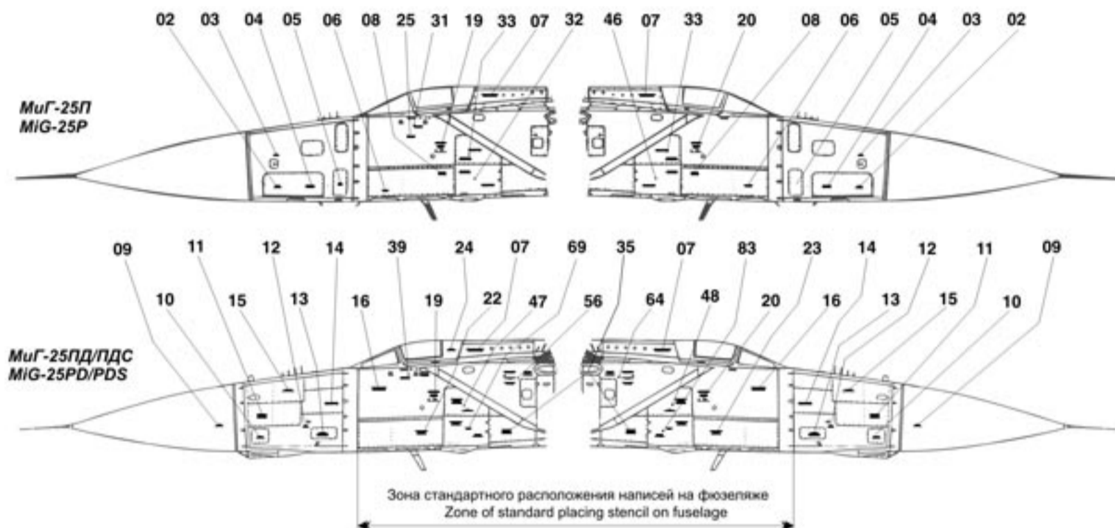
Nose parts of fuselage from MiG-25 various modifications
